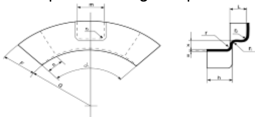
C、保护正角环片 Protections to Angle Rings
